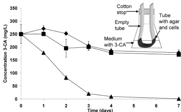
FIGURE 2. Concentration of 3-CA in the diffusion-mediated degradation experiment: control without cells (◆); agar-embedded I2gfp cells (▲); agar-embedded E. coli cells (■). Values represent the mean \pm error bars ( n = 2 ); in some cases, the standard deviations were too small to be visible. A representation of the experimental setup is shown beside the graph.
